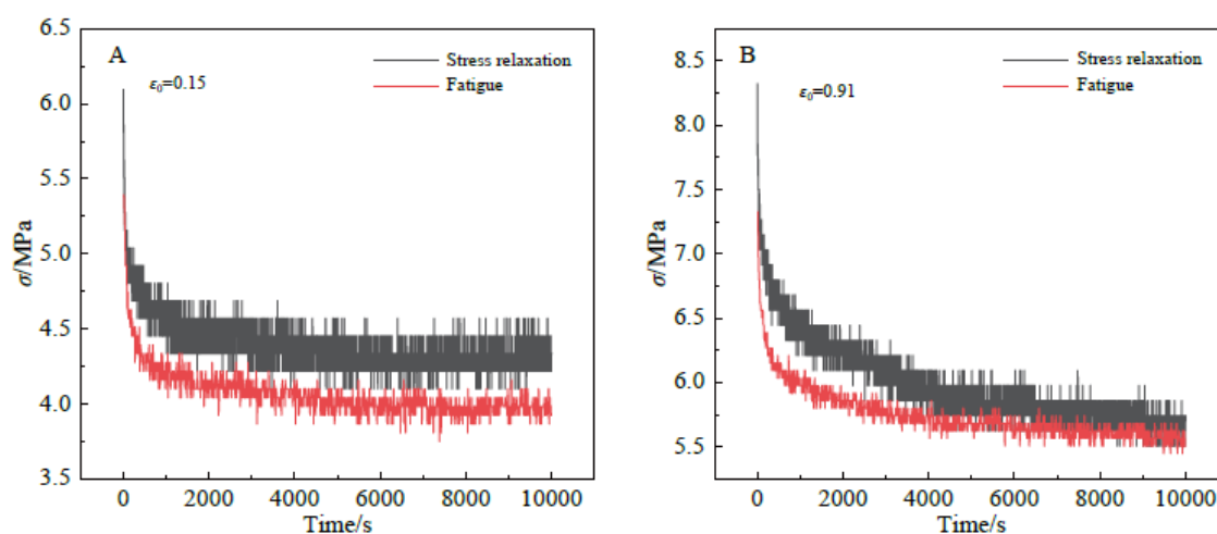
Fig. 4 Stress decay profiles of the sample during stress relaxation and fatigue testing with pre-strain levels of 0.15 (A) and 0.91 (B)
