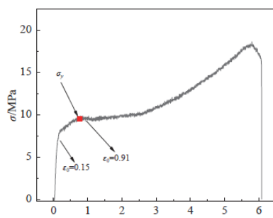
Fig. 2 Engineering stress-strain curve of the sample. The red dot represents the yield point. Two pre-strain values of 0.15 and 0.91 were selected to conduct the subsequent stress relaxation and fatigue measurements
